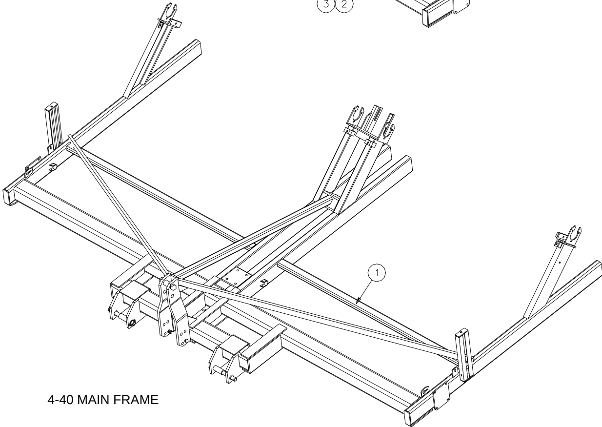
4-31, 4-36, & 4-38 MAIN FRAME
