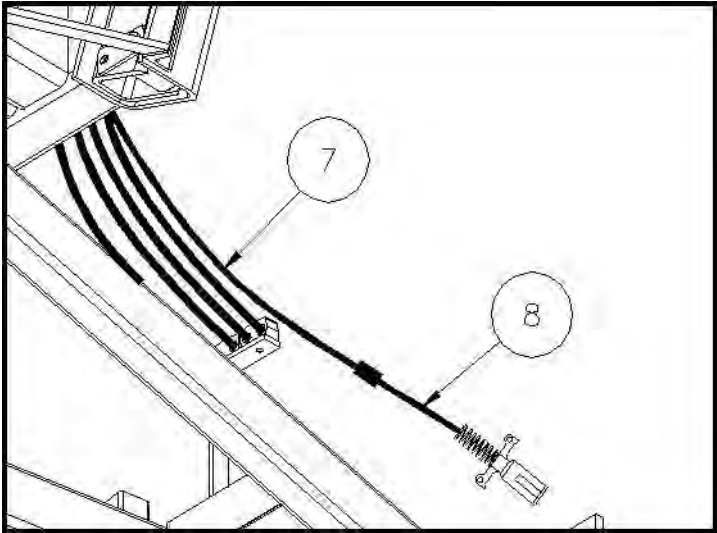
TONGUE WITH WIRING HARNESS AND 7-WAY PLUG ADAPTER.
