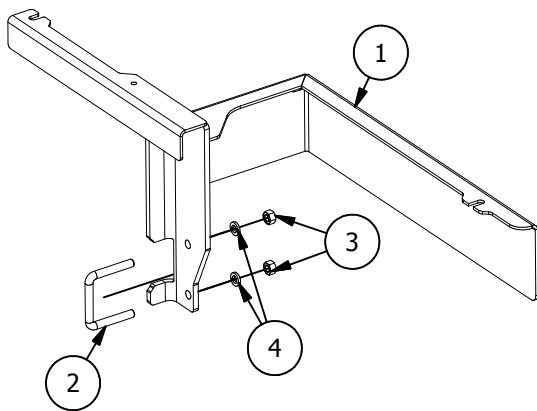
BREAKDOWN OF: 21-082-148 LIGHT BRACKET ASSY, LT
