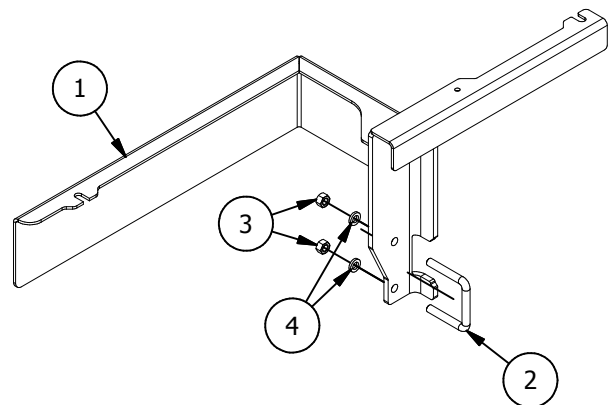
BREAKDOWN OF: 21-082-149 LIGHT BRACKET ASSY, RT
