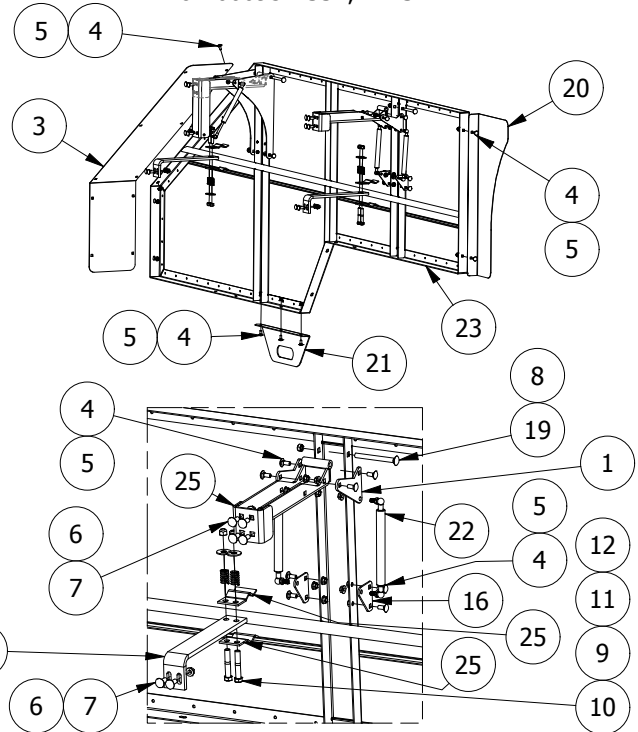
74-181-00093 ASSY, RT SHIELD
