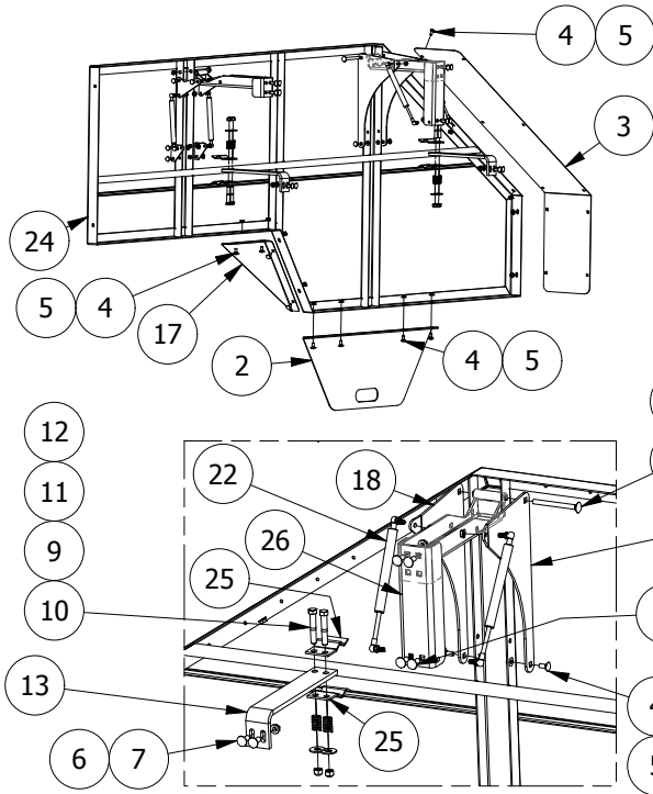
74-181-00094 ASSY, LT SHIELD
