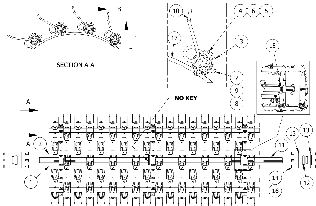
DETAIL B
