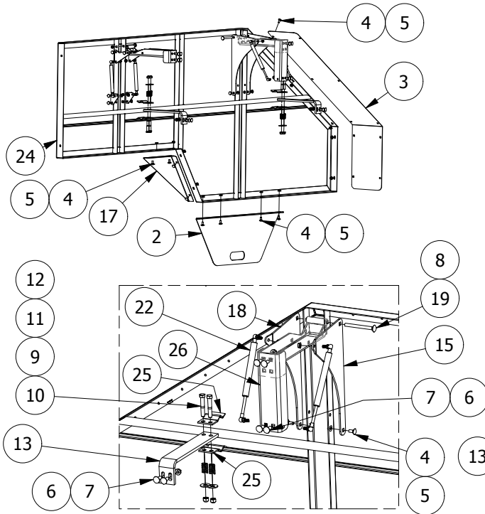
74-181-00094 ASSY, LT SHIELD
